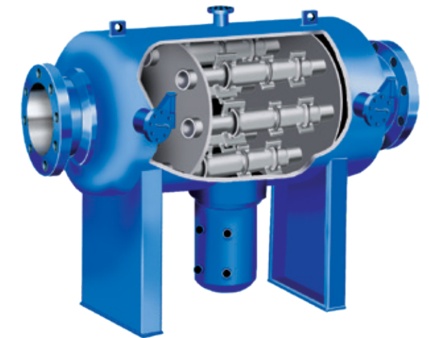
Series 95H-CT Separator
